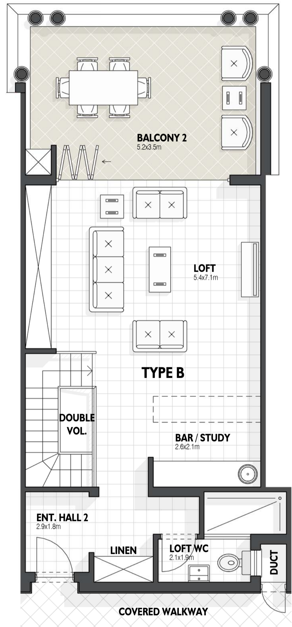
LOFT PLAN (SECOND STOREY)
